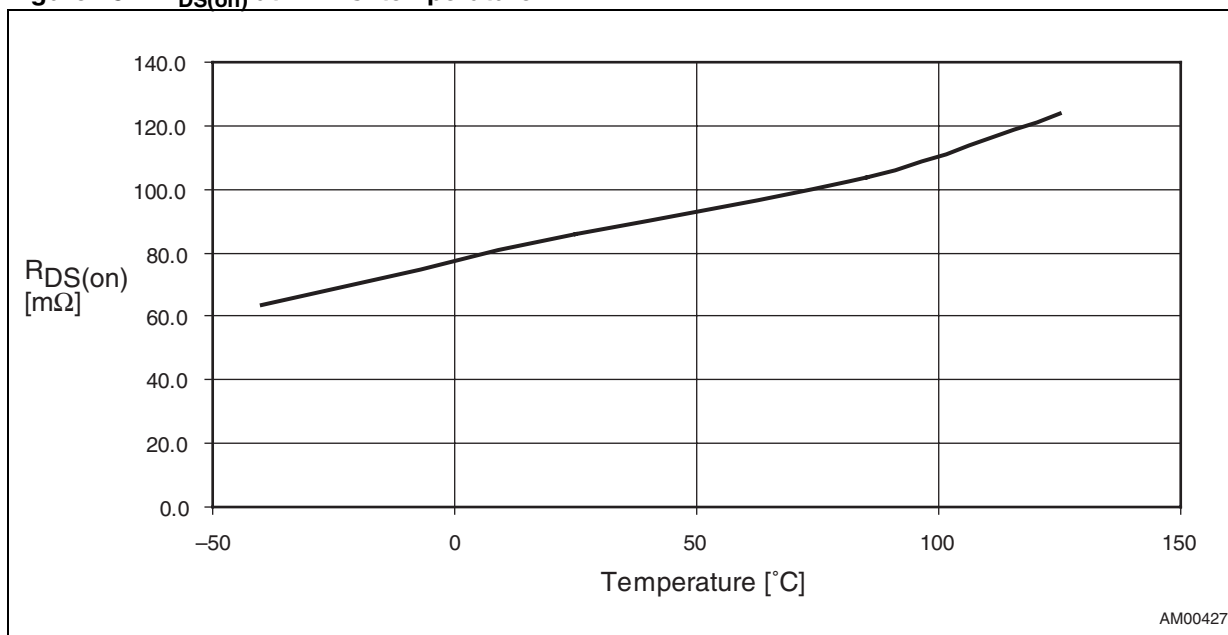
Figure 25. R_{DS(on)} at 1 A vs. temperature
