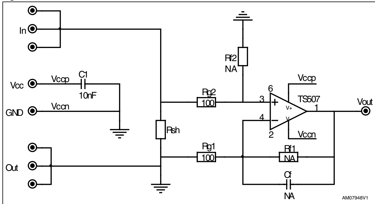
Figure 1. Internal schematic
