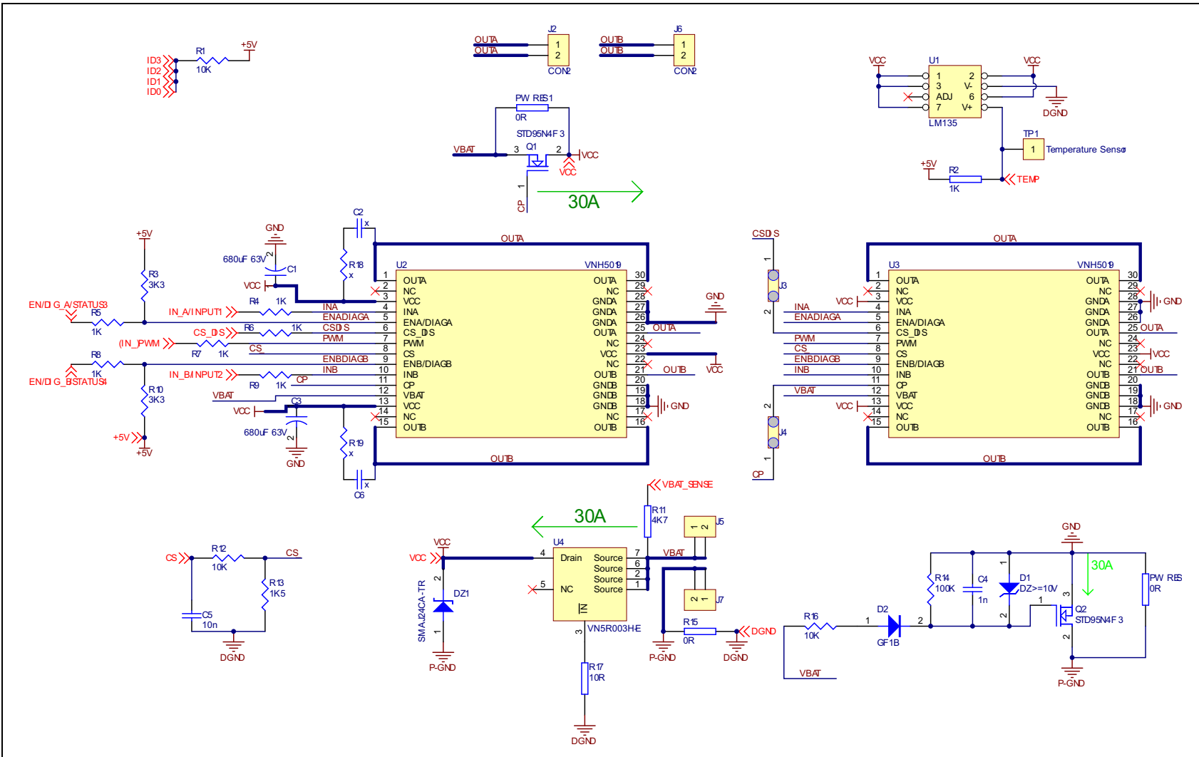
Figure 4. VN5019A daughterboard application schematic (part 2)
