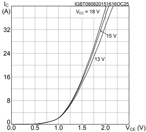
Figure 9. Output characteristics
