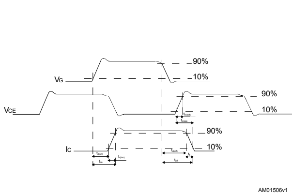
Figure 29. Switching waveform
