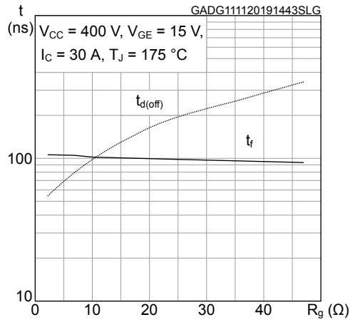
Figure 19. Switching times vs gate resistance
