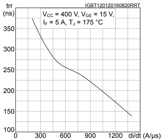
Figure 21. Reverse recovery time vs diode current slope
