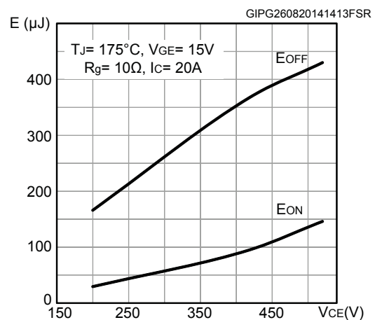
Figure 18. Switching energy vs collector emitter voltage
