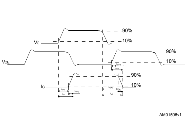
Figure 27. Switching waveform
