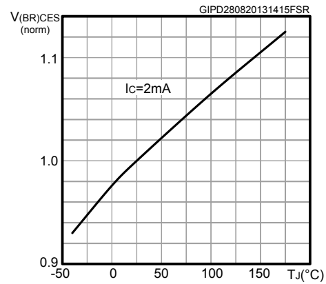
Figure 10. Normalized V_{(BR)CES} vs junction temperature
