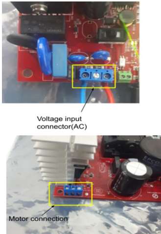
Figure 6. Voltage Input and Motor Connection
