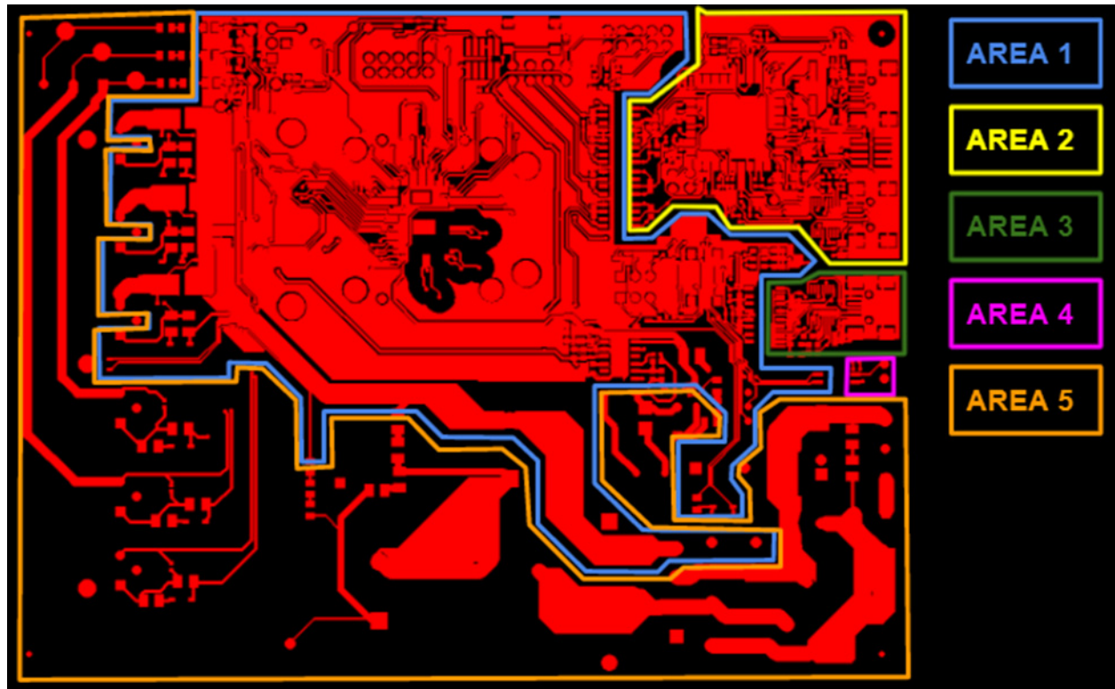
Figure 3. Voltage Map
