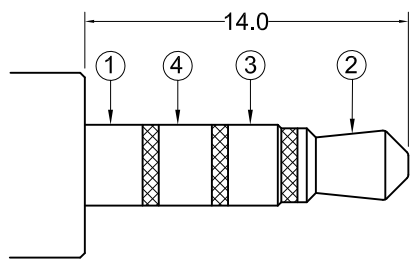
Ø3.5 MATE PLUG
