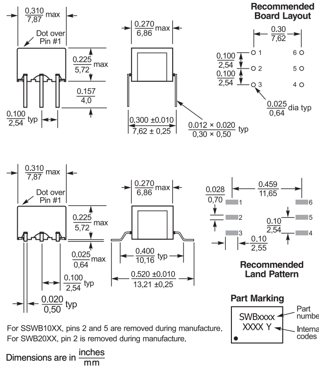
SWB1010-1, SWB2010-1, SWB3010-1 3 dB bandwidth 0.04 – 175 MHz
