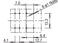
Mounting Hole Layout
