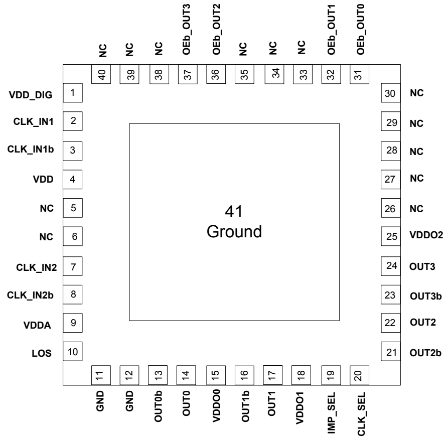
Figure 6.4. Si53254A-D02AM 40-QFN
