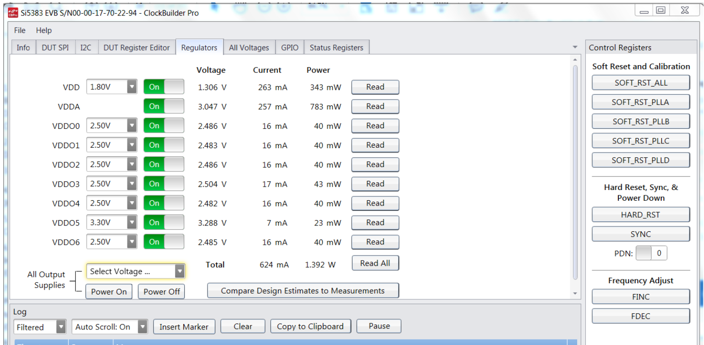
Figure 6.3. EVB GUI
