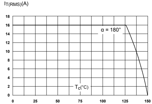
Figure 2. On-state RMS current versus case temperature
