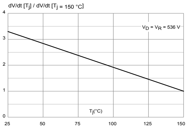
Figure 13. Relative variation of static dV/dt immunity versus junction temperature
