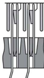
Yamaichi's 2-point Tweezer Style Contact
