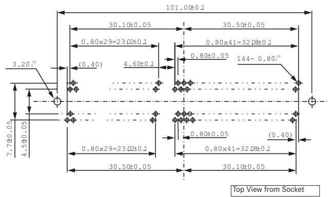
Top View from Socket
