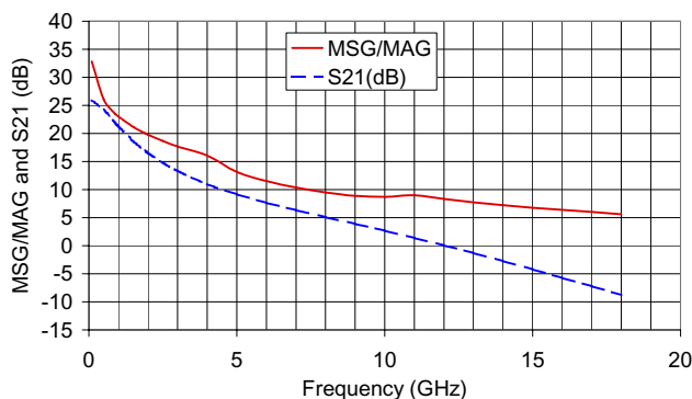
MAXIMUM STABLE GAIN (MSG)/MAXIMUM AVAILABLE GAIN (MAG) vs. FREQUENCY V_{DS}=3V & I_{DS}=20mA
