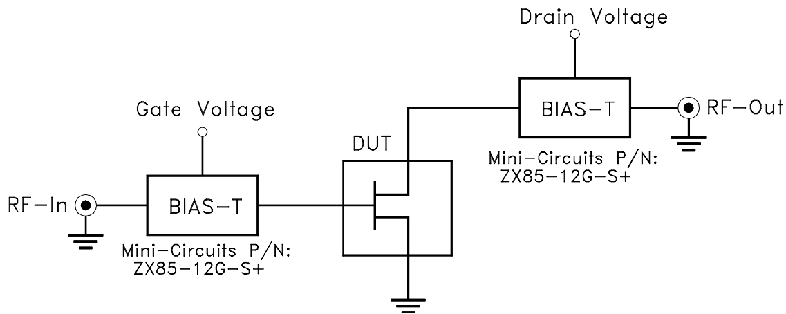
Fig 1. Block Diagram of Test Circuit used for characterization. (DUT soldered on Mini-Circuits Test Board TB-154 Gain, Output power at 1dB compression (P1 dB) and output IP3 (OIP3) are measured using R&S Network Analyzer ZVA-24. Noise Figure measured using Agilent's Noise Figure meter N8975A and noise source N4000A.
