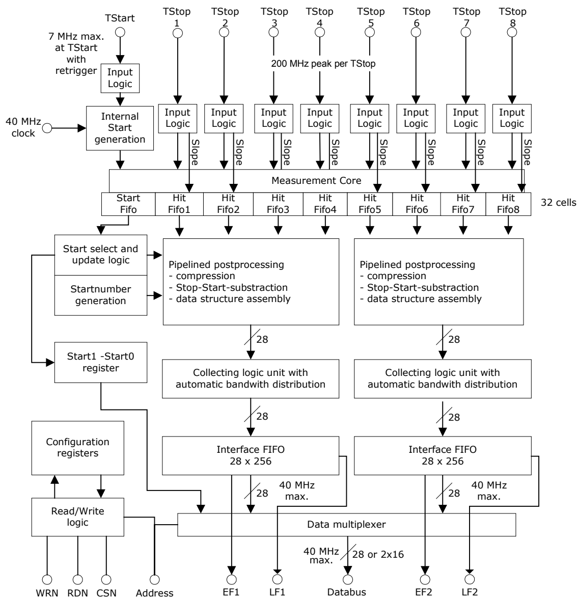
Figure 16: Block diagram
