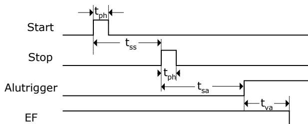
Figure 35: Measurement timings
