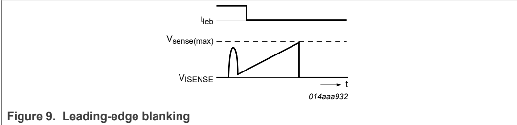
Figure 9. Leading-edge blanking
