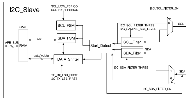
Figure 52: I2C Slave Architecture
