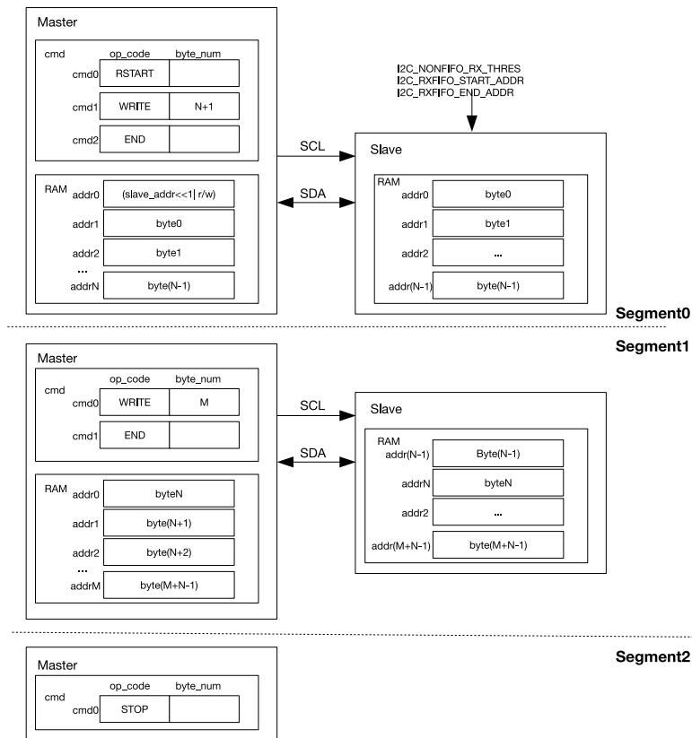
Figure 58: Master Writes to Slave with 7-bit Address in Three Segments
