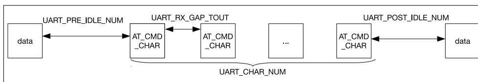
Figure 85: AT_CMD Character Format
