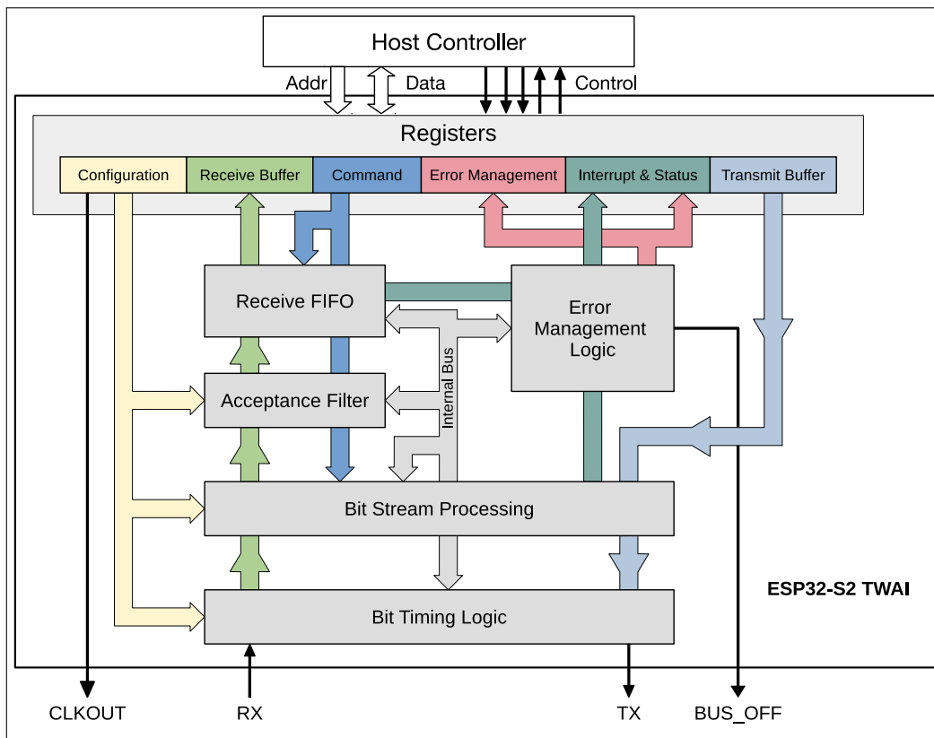
Figure 131: TWAI Overview Diagram
