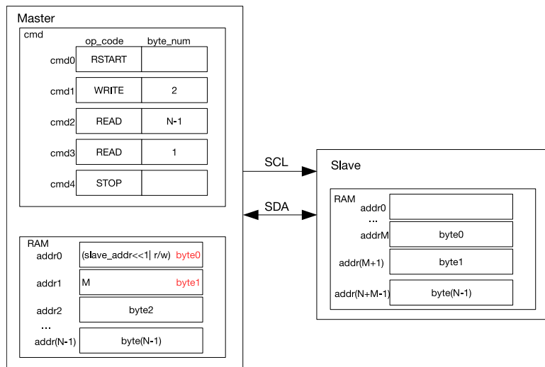
Figure 61: Master Reads N Bytes of Data from addrM in Slave with 7-bit Address
