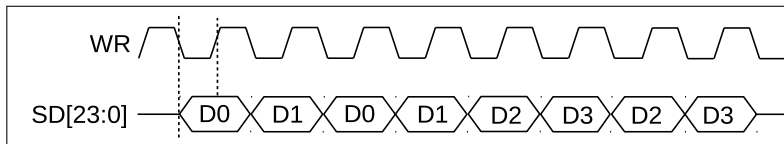
Figure 77: LCD Master Transmitting Data Frame, Form 2
