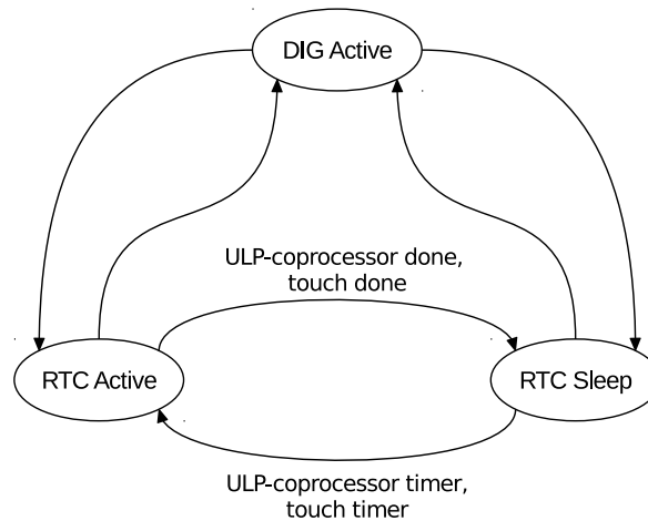
Figure 182: RTC States
