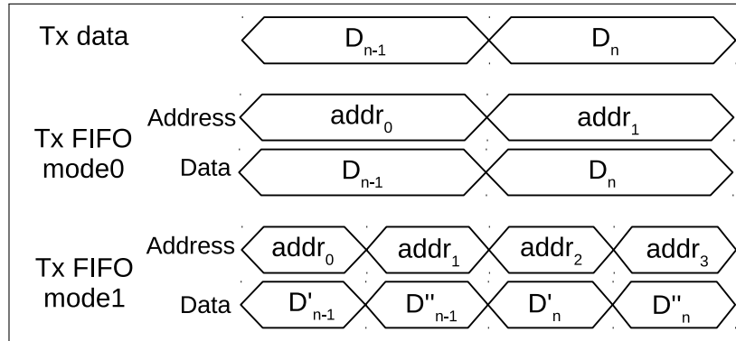
Figure 68: Tx FIFO Data Mode
