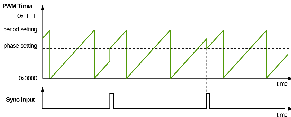
Figure 100: Count-Up Mode Waveform
