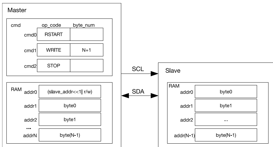
Figure 55: I2C Master Writes to Slave with 7-bit Address
