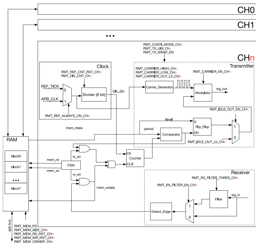
Figure 92: RMT Architecture
