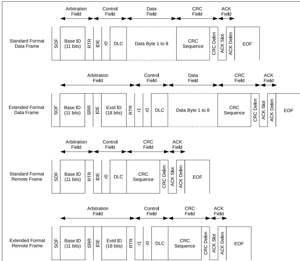
Figure 126: The bit fields of Data Frames and Remote Frames
