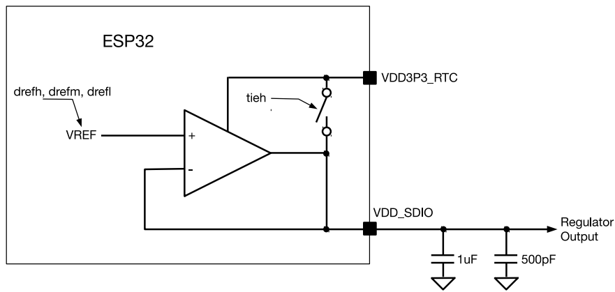
Figure 177: Flash Voltage Regulator
