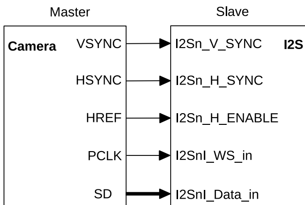
Figure 78: Camera Slave Receiving Mode
