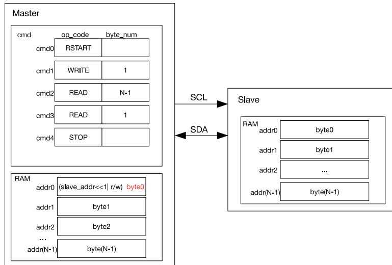
Figure 59: Master Reads from Slave with 7-bit Address
