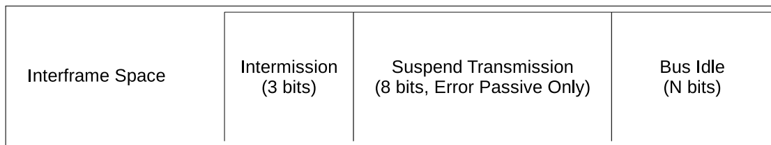
Figure 129: The Fields within an Interframe Space
