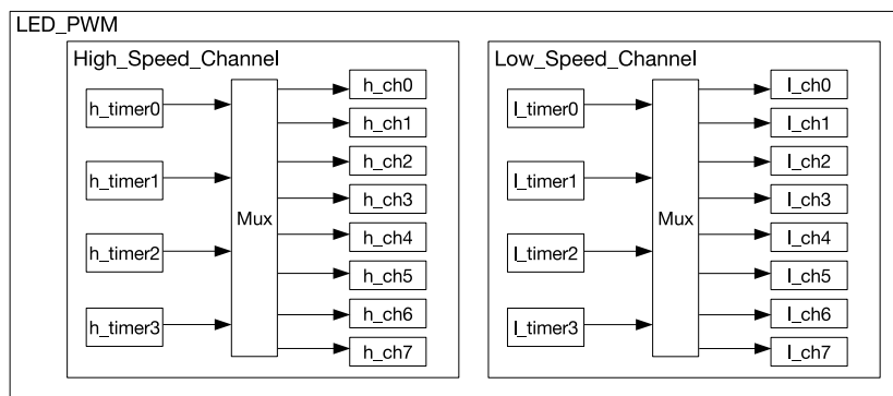
Figure 87: LED_PWM Architecture
