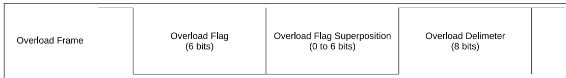
Figure 128: The Bit Fields of an Overload Frame
