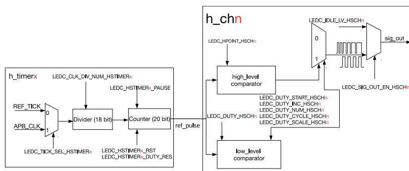
Figure 88: LED_PWM High-speed Channel Diagram
