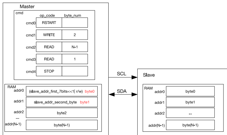
Figure 60: Master Reads from Slave with 10-bit Address
