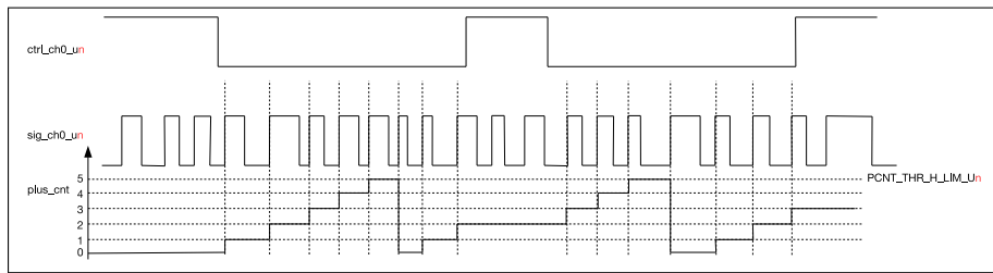
Figure 124: PULSE_CNT Upcounting Diagram
