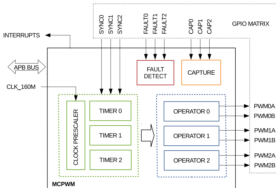
Figure 94: MCPWM Module Overview
