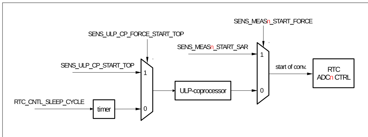
Figure 147: RTC SAR ADC Outline of Function
