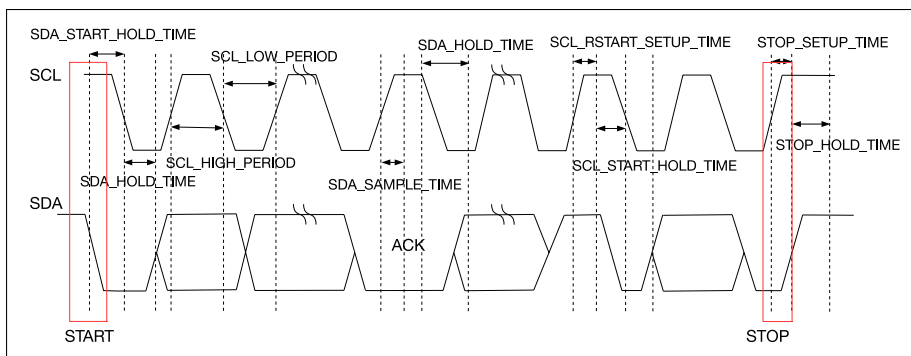
Figure 53: I2C Sequence Chart
