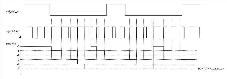
Figure 125: PULSE_CNT Downcounting Diagram
