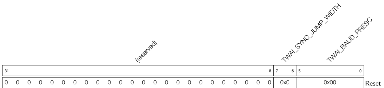
Register 21.2: TWAI_BUS_TIMING_0_REG (0x0018)
