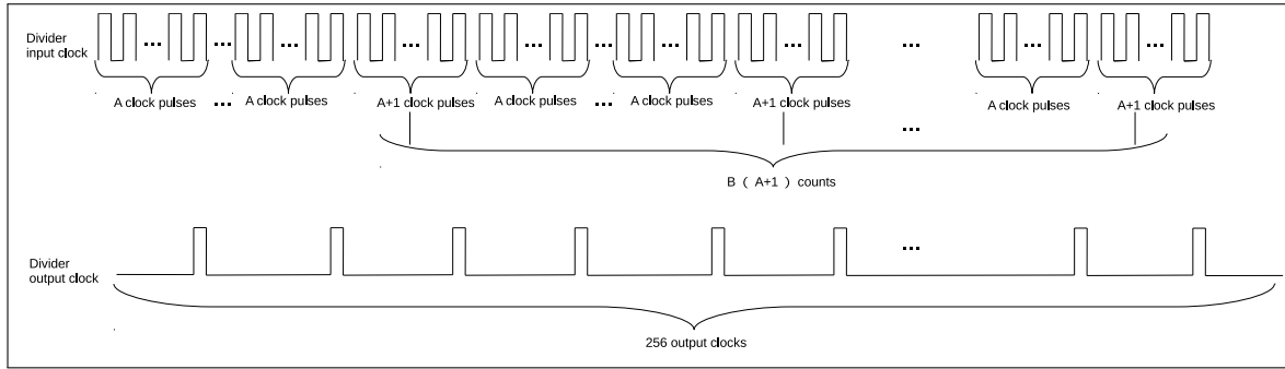
Figure 89: LED_PWM Divider
