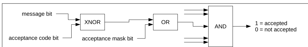
Figure 132: Acceptance Filter
