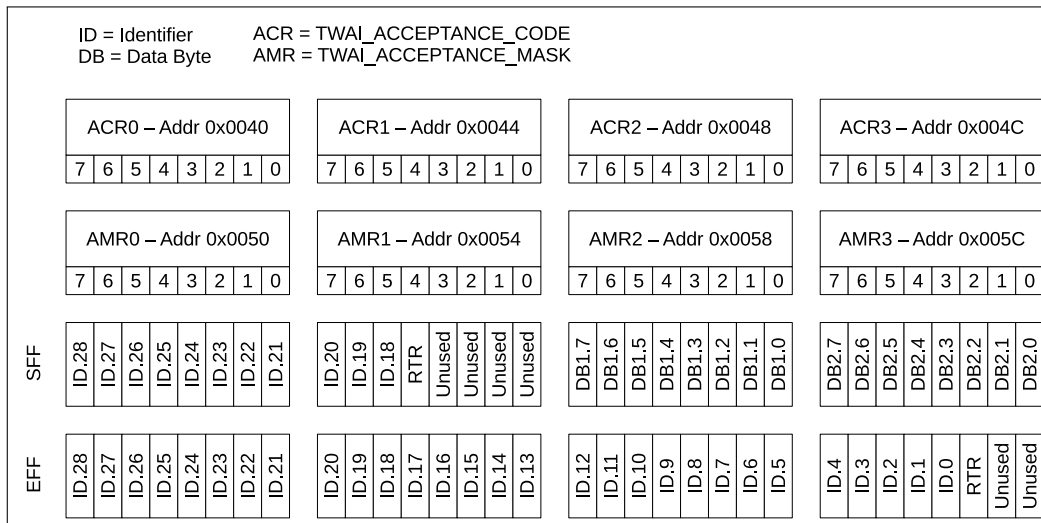
Figure 133: Single Filter Mode
