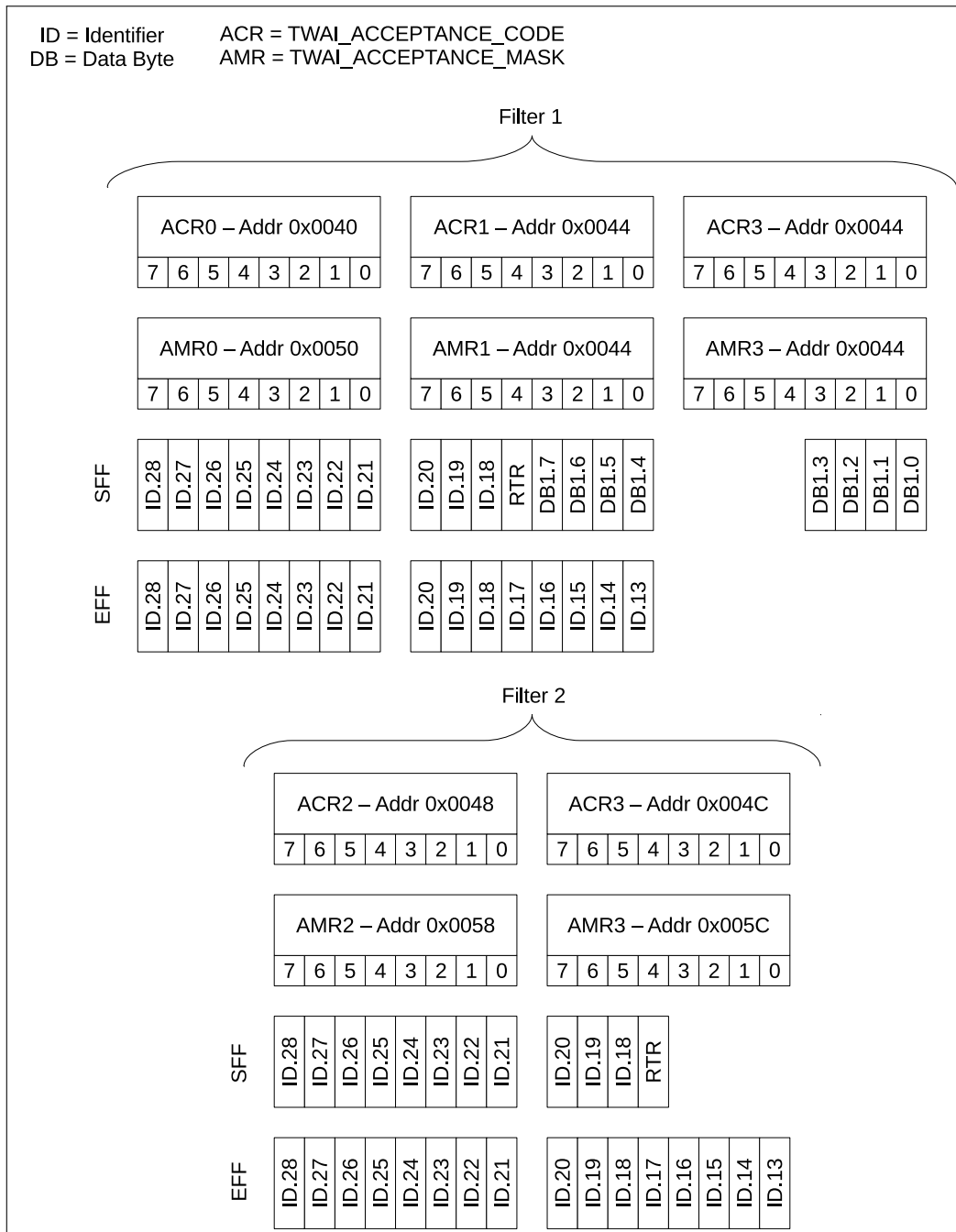
Figure 134: Dual Filter Mode
