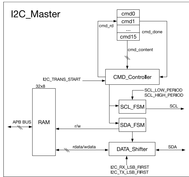
Figure 51: I2C Master Architecture
