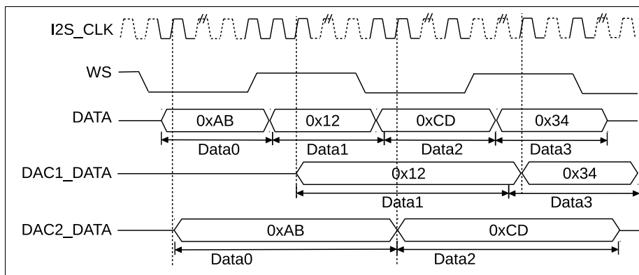
Figure 81: Data Input by I2S DAC Interface
