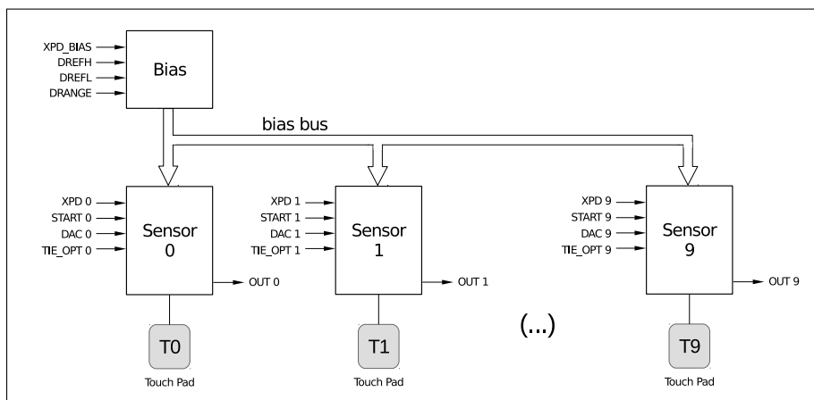
Figure 142: Touch Sensor Structure
