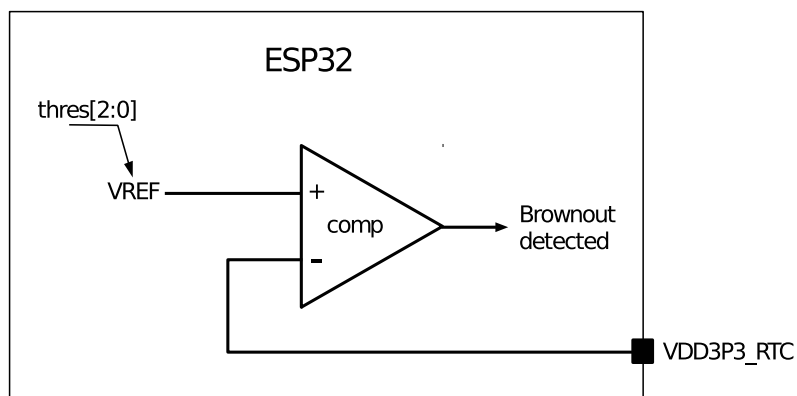
Figure 178: Brownout Detector
