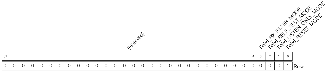
Register 21.1: TWAI_MODE_REG (0x0000)
