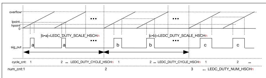
Figure 91: Output Signal Diagram of Fading Duty Cycle
