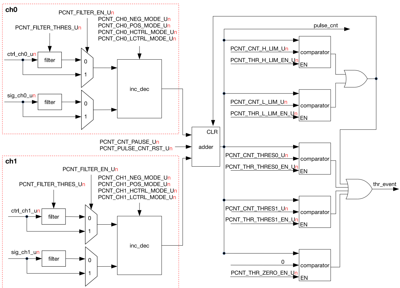
Figure 123: PULSE_CNT Architecture
