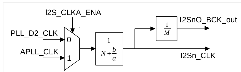
Figure 64: I2S Clock
