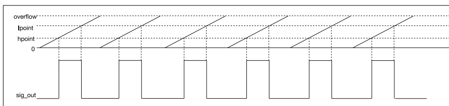
Figure 90: LED PWM Output Signal Diagram
