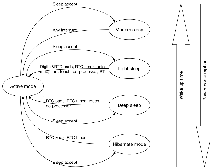
Figure 183: Power Modes
