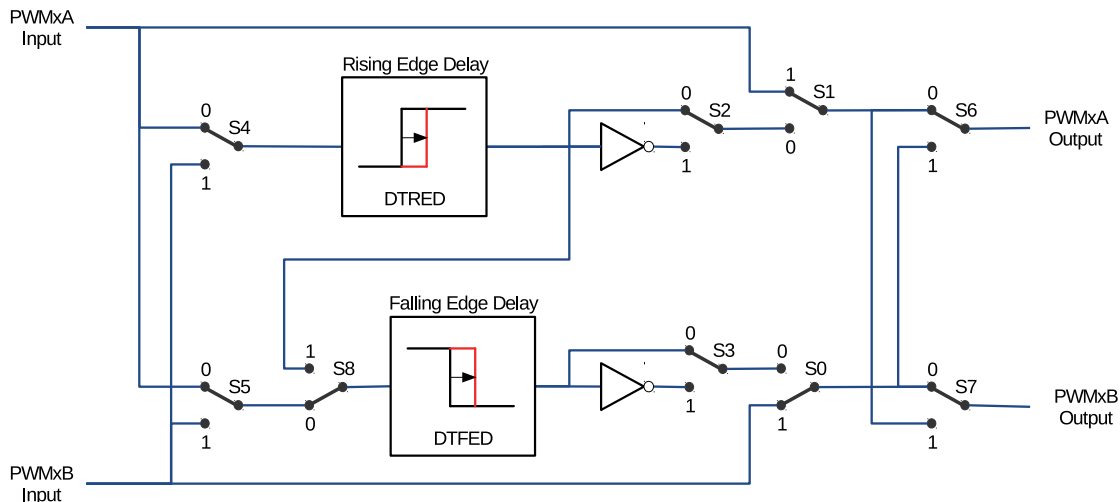
Figure 115: Options for Setting up the Dead Time Generator Submodule
