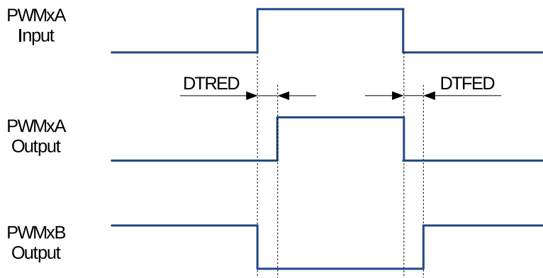
Figure 116: Active High Complementary (AHC) Dead Time Waveforms
