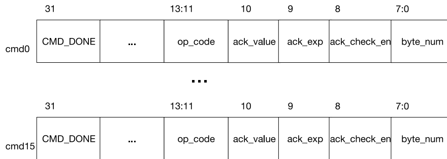
Figure 54: Structure of The I2C Command Register
