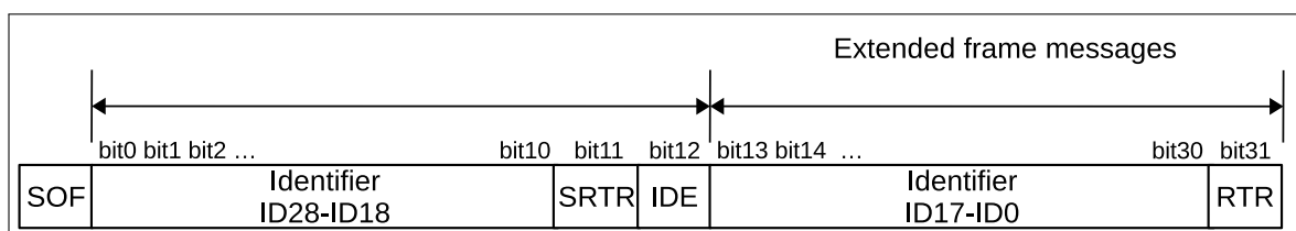
Figure 136: Positions of Arbitration Lost Bits
