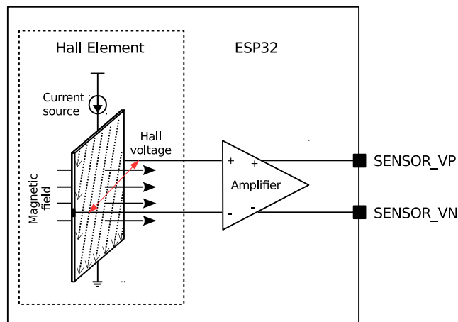
Figure 149: Hall Sensor
