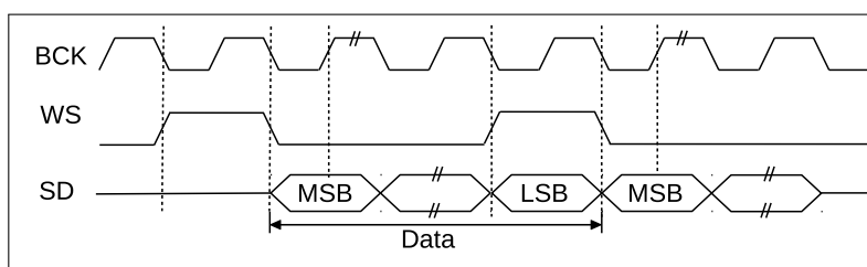
Figure 67: PCM Standard
