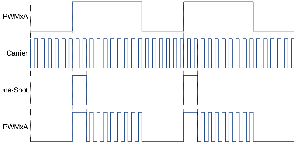
Figure 121: Example of the First Pulse and the Subsequent Sustaining Pulses of the PWM Carrier Submodule
