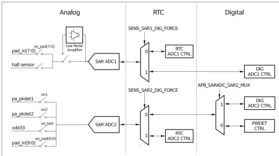
Figure 146: SAR ADC Outline of Function
