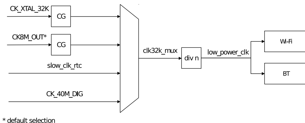
Figure 181: Digital Low-Power Clocks
