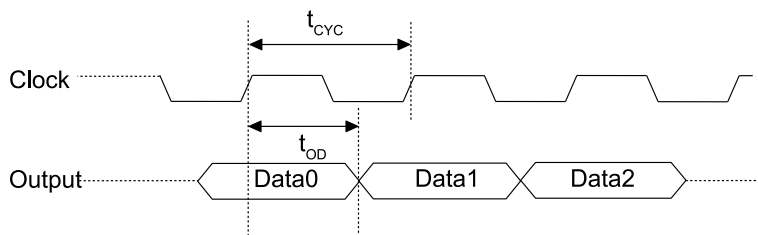
Figure 48: RMIITransmitting Data
