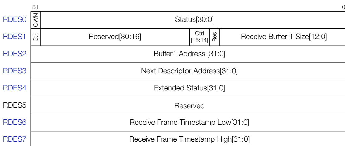
Figure 50: Receive Descriptor
