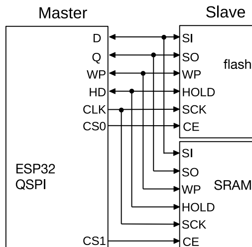
Figure 20: Parallel QSPI
