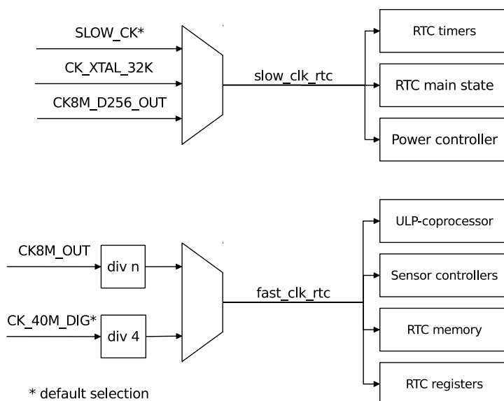
Figure 180: RTC Low-Power Clocks
