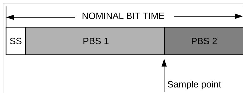
Figure 130: Layout of a Bit
