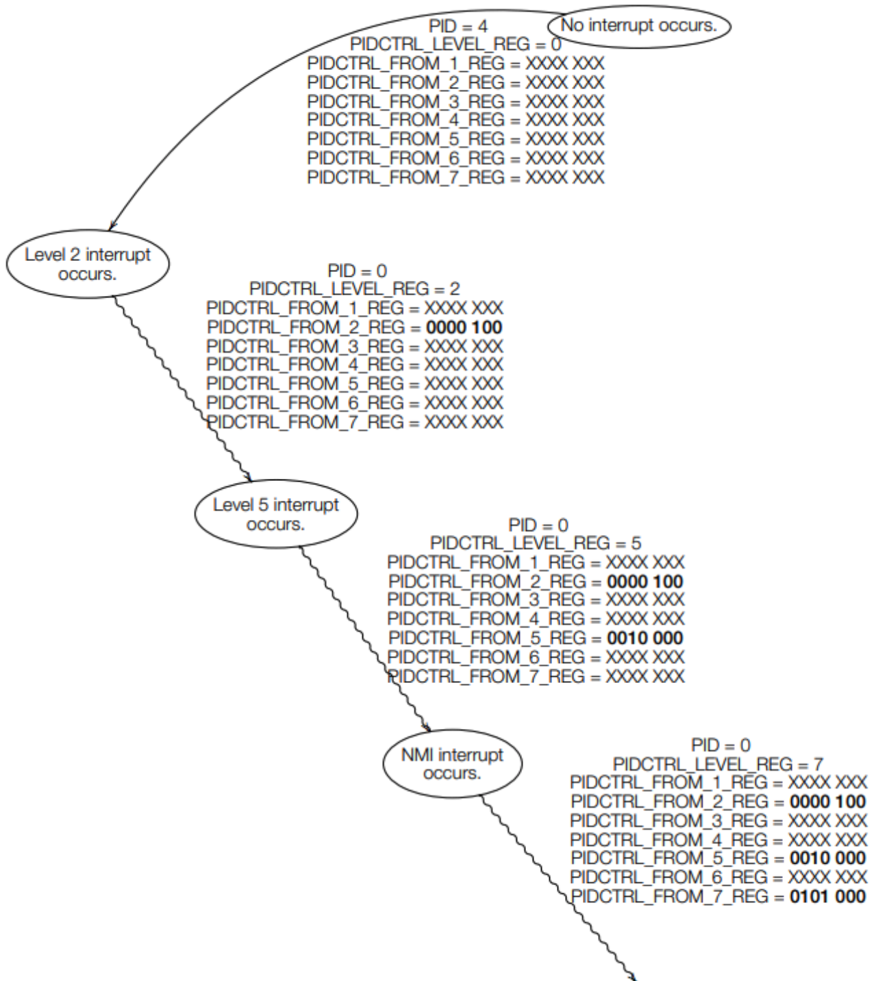
Figure 140: Interrupt Nesting
