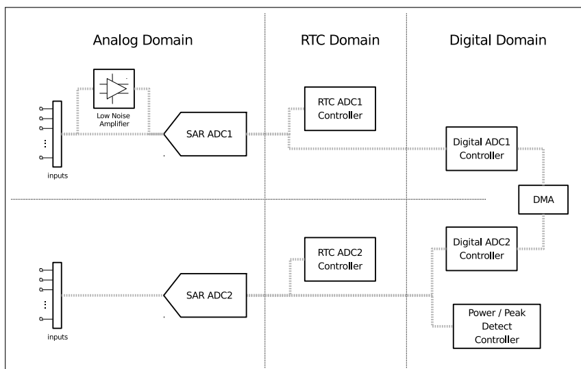
Figure 145: SAR ADC Depiction
