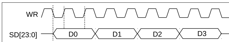
Figure 76: LCD Master Transmitting Data Frame, Form 1
