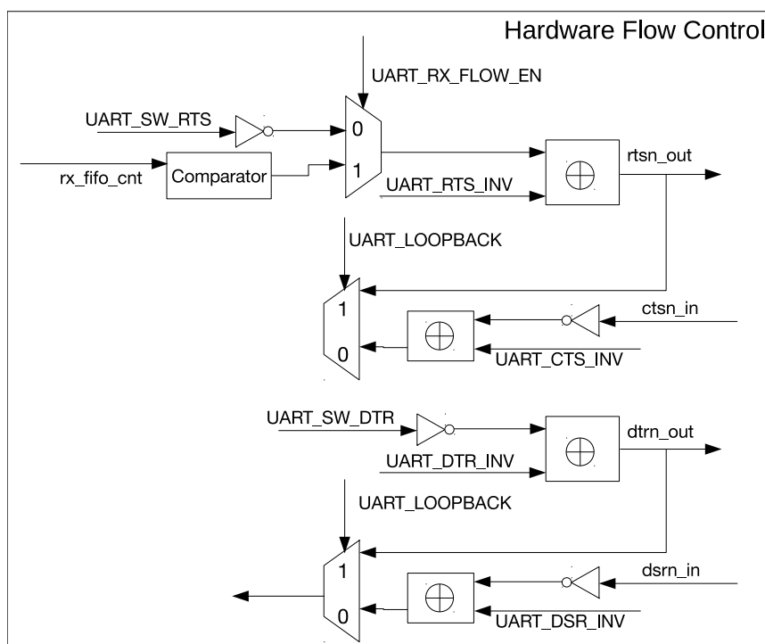
Figure 86: Hardware Flow Control
