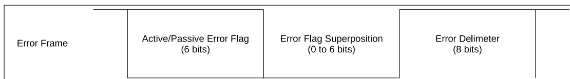
Figure 127: Various Fields of an Error Frame
