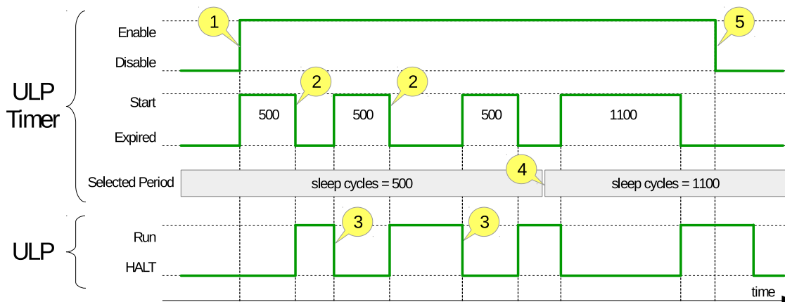
Figure 171: Sample of a ULP Operation Sequence
