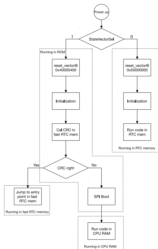
Figure 184: ESP32 Boot Flow
