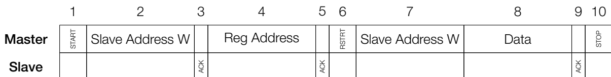
Figure 173: I 2 C Write Operation
