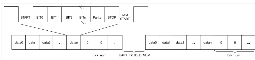
Figure 84: UART Data Frame Structure
