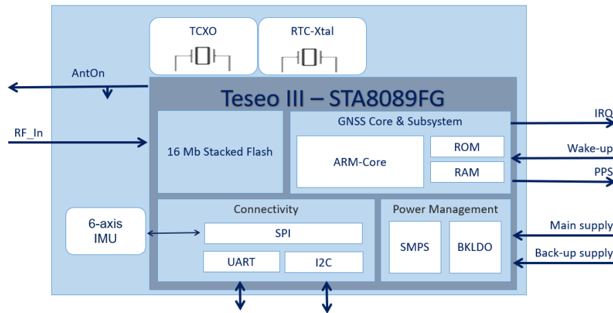
Figure 1. Block schematic
