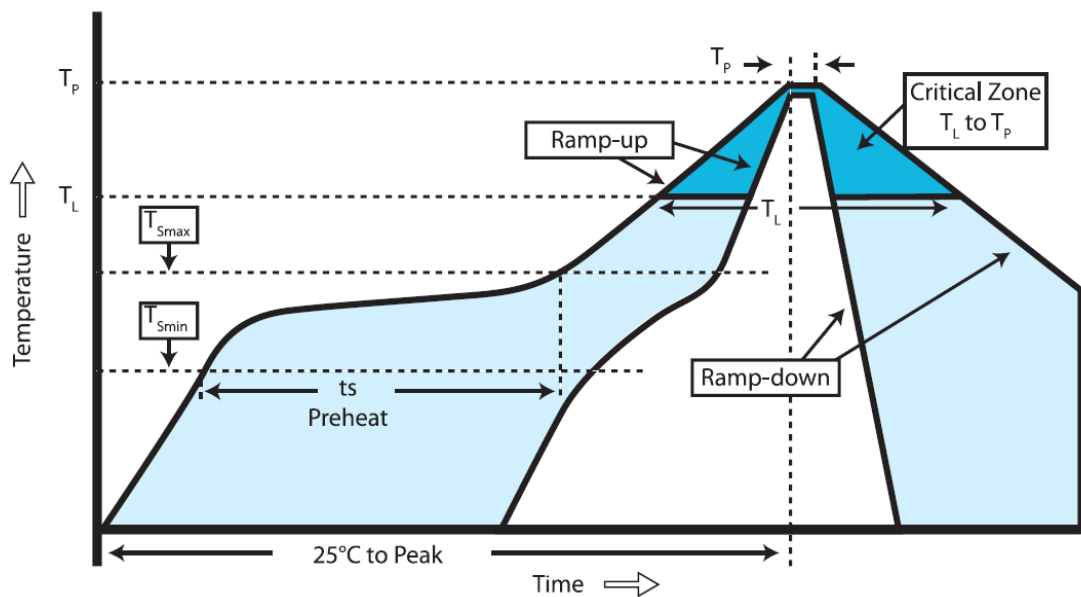
Figure 10. Soldering profile
