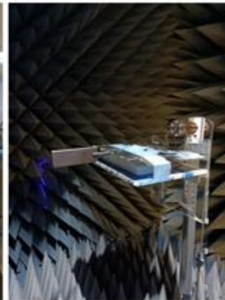
Chamber & VNA setup straight on the edge of a 30x30cm ground plane
