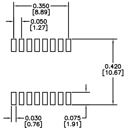
RECOMMENDED SOLDER PAD DIMENSIONS
