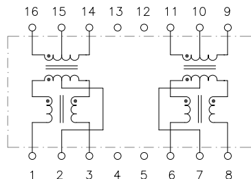
Circuit A
