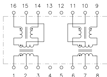
Circuit C
