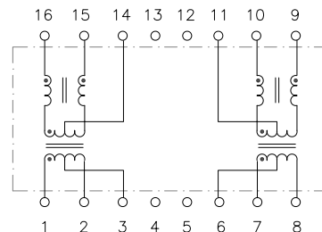
Circuit B
