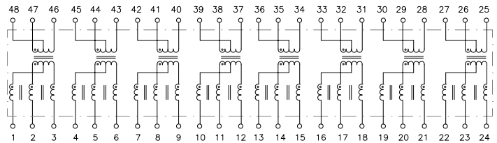
Circuit D
