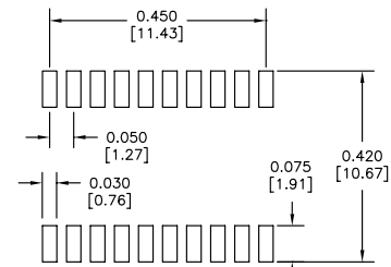
Recommended Solder Pad Layout
