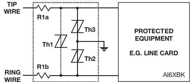
Figure 15. Protection Module
