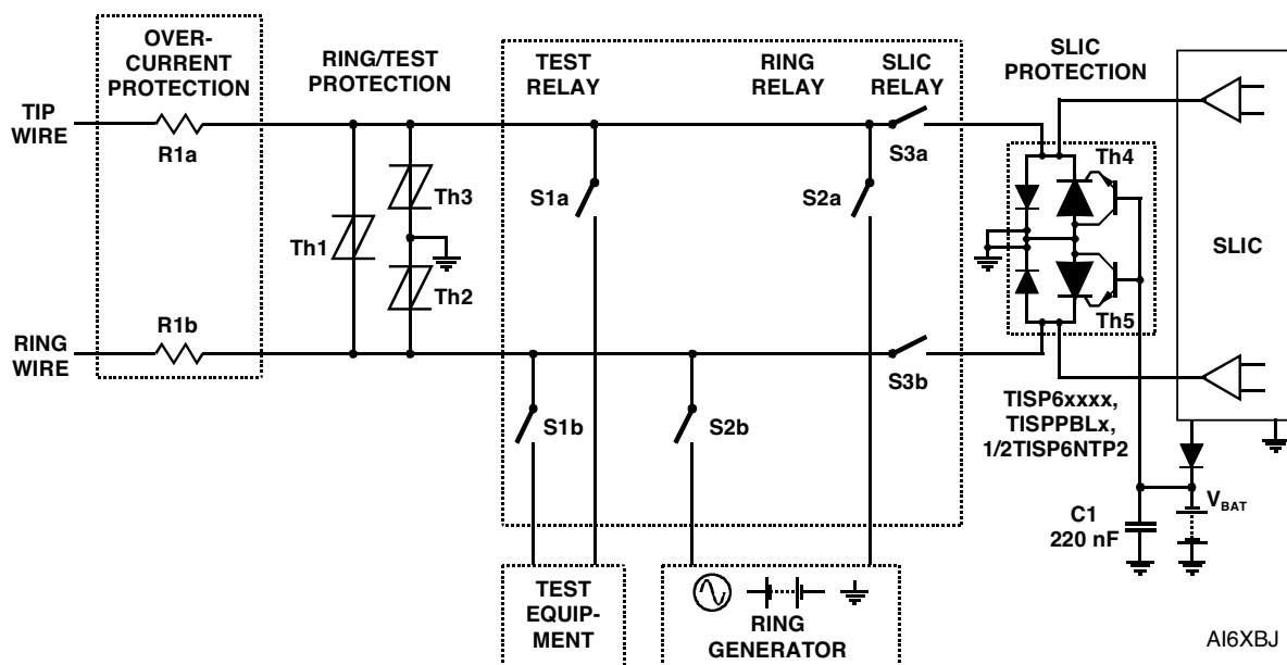
Figure 17. Line Card Ring/Test Protection
