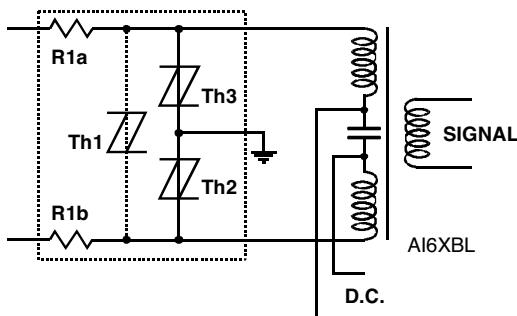
Figure 16. ISDN Protection
