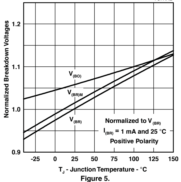
NORMALIZED BREAKDOWN VOLTAGES vs JUNCTION TEMPERATURE
