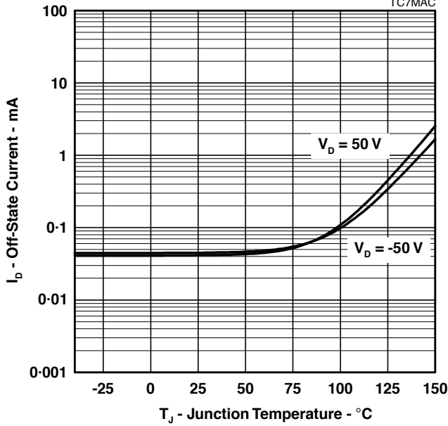
TISP7125F3 THRU TISP7180F3 OFF-STATE CURRENT vs JUNCTION TEMPERATURE
