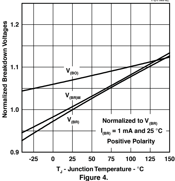
NORMALIZED BREAKDOWN VOLTAGES vs JUNCTION TEMPERATURE
