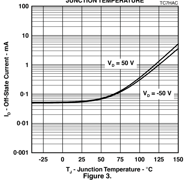
TISP7240F3 THRU TISP7380F3 OFF-STATE CURRENT vs JUNCTION TEMPERATURE
