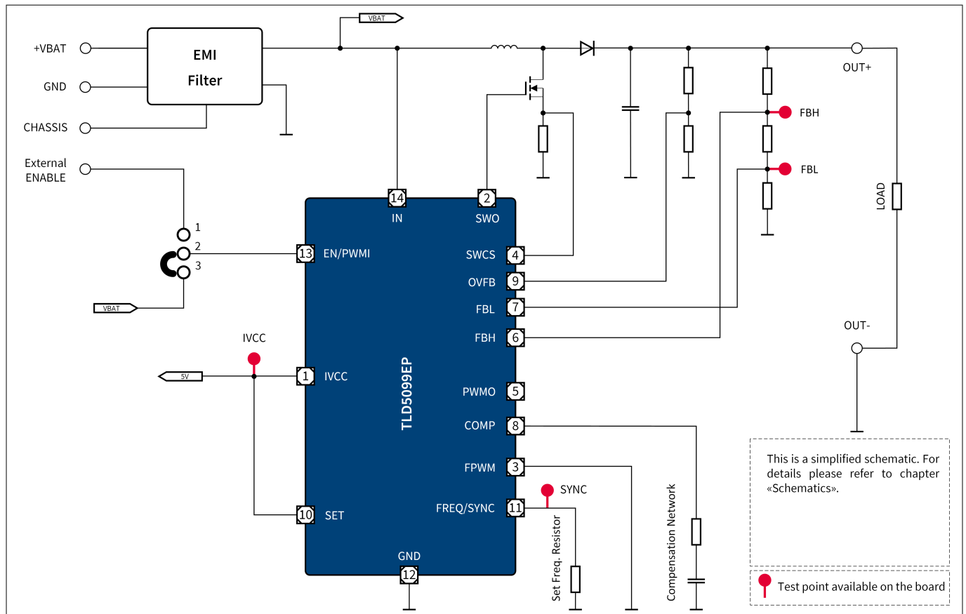
Figure 2 Simplified schematic
