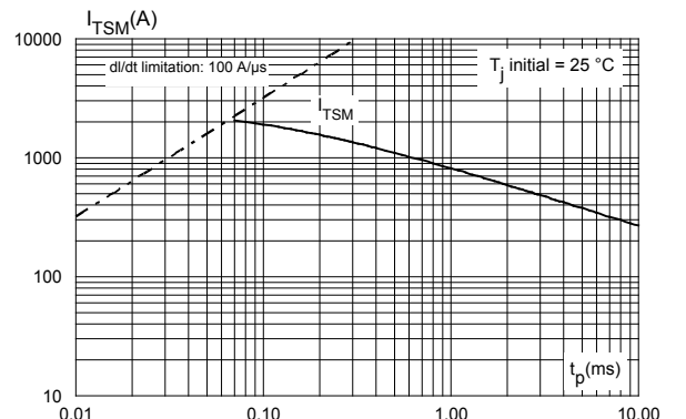
Figure 10. Non repetitive surge peak on-state current for a sinusoidal pulse with width t_p < 10 ms
