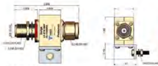
• LP-BTR-NMP 20-1000MHz DC Blocked N Type M on Protected
