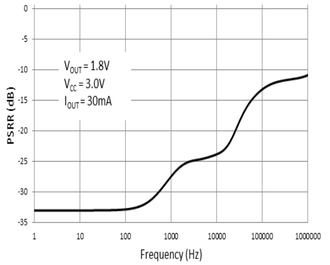
Power Supply Rejection Ratio
