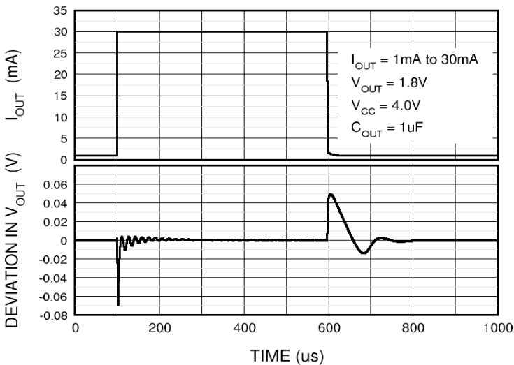
Load Step Response
