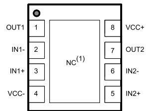
DFN8 2x2
