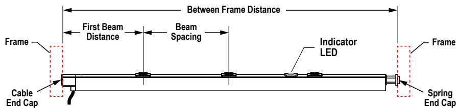
Figure 2. T-Slot Configuration
