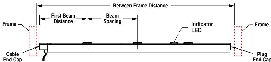
Figure 2. T-Slot Configuration
