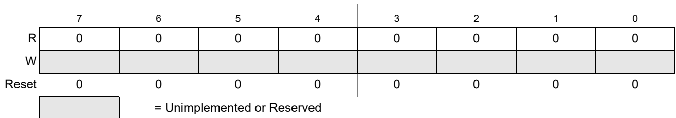
Figure 29-24. Flash Reserved6 Register (FRSV6)
