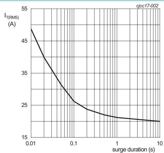
Fig. 2. RMS on-state current as a function of surge duration; maximum values f = 50\text{ Hz} ; T_{mb} = 116\text{ °C}
