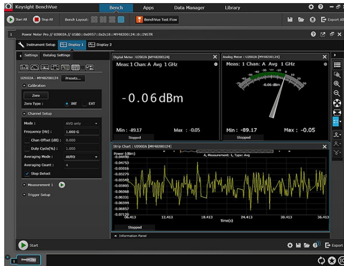
Digital meter, analog meter and datalog view.
