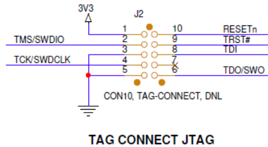
Figure 4 – Tag-Connect JTAG adapter, cables, and pinout for 10-pin TC2050
