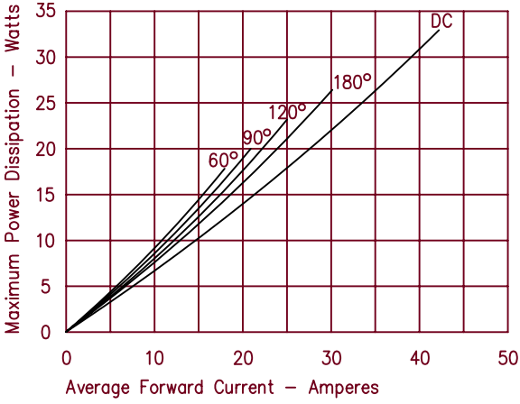
Figure 7 Maximum Forward Power Dissipation – Reverse Polarity
