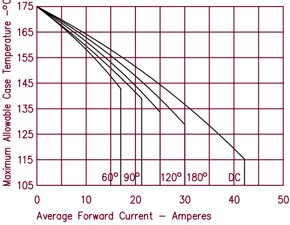
Figure 6 Forward Current Derating – Reverse Polarity
