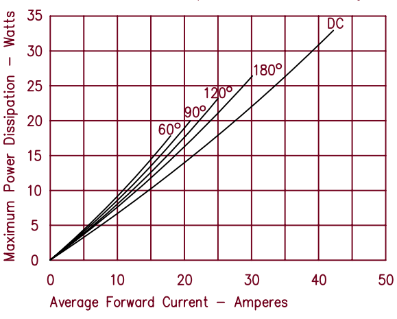
Figure 7 Maximum Forward Power Dissipation – Reverse Polarity
