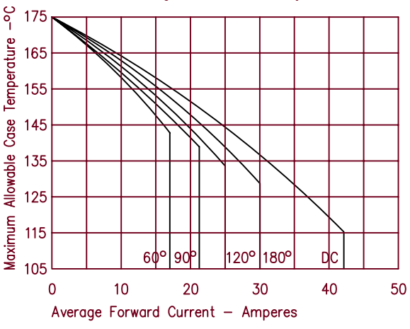
Figure 6 Forward Current Derating – Reverse Polarity
