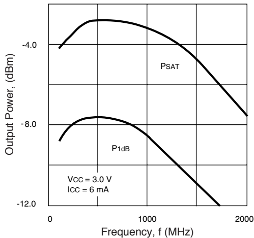
UPC2748TB POWER vs. FREQUENCY
