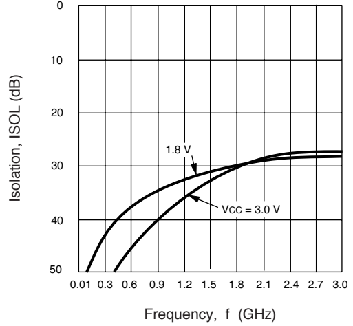
UPC2747TB ISOLATION vs. FREQUENCY
