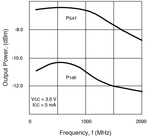
UPC2747TB POWER vs. FREQUENCY
