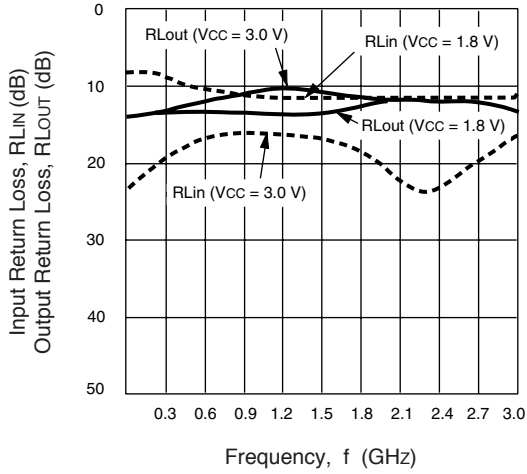
UPC2747TB RETURN LOSS vs. FREQUENCY
