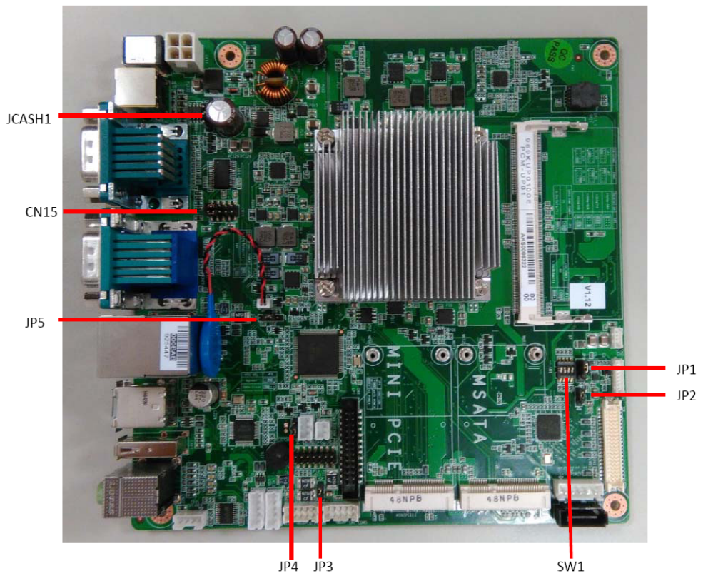
Figure 3.1 Jumper Locations
