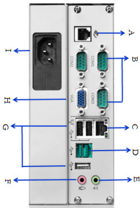
Figure 2.3 I/O interface
