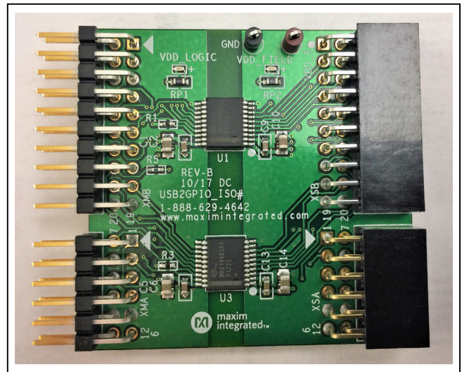
Figure 1. USB2GPIOISO# Board
