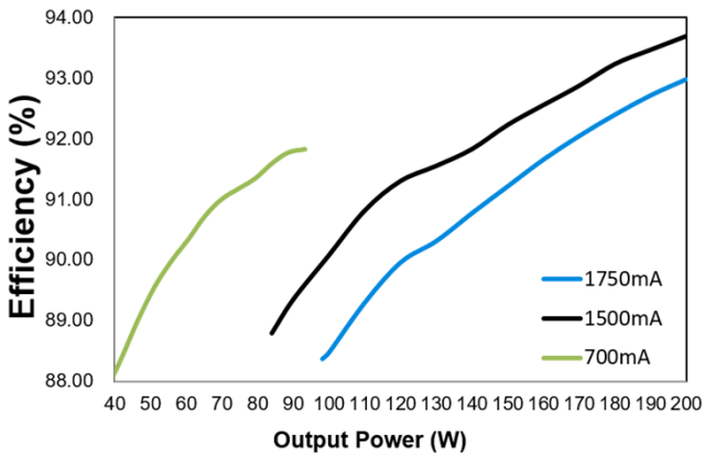
Efficiency @ 277Vac
