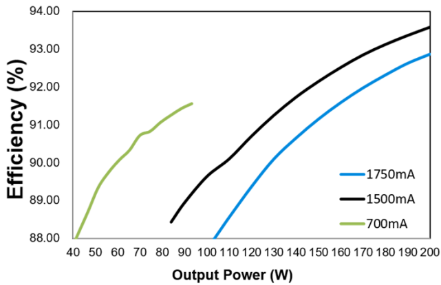
Efficiency @ 230Vac
