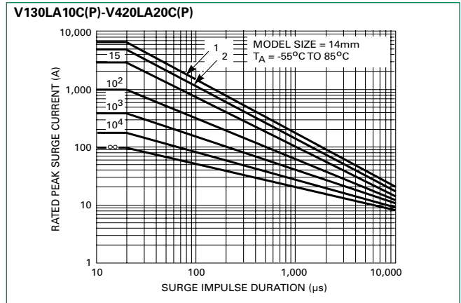
Figure 6. Repetitive Surge Capability for 14mm Parts
